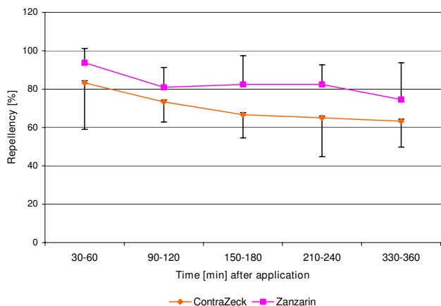
Figure 2 Test in humans [A]. Relative repellency of ContraZeck® and Zanzarin® against I. ricinus nymphs. Each data point in the graph is the mean ± S.D. of relative repellency (with respect to the controls) in six volunteers and of 12 nymphs tested in each volunteer (n = 72) at the respective time interval.
