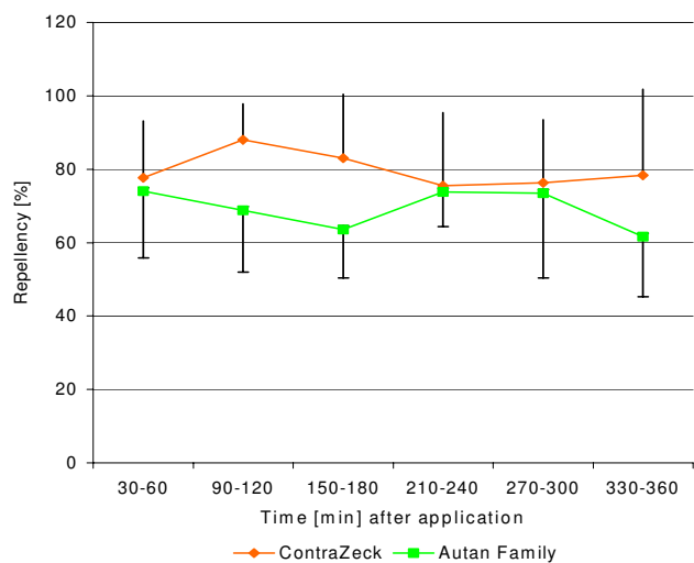
Figure 3 Test in humans [B]. Relative repellency of ContraZeck® and Autan® Family against adult I. ricinus ticks. Each data point in the graph is the mean \pm S.D. of relative repellency (with respect to the controls) in six volunteers and of 12 adult ticks tested in each volunteer ( n = 72 ) at the respective time interval.
